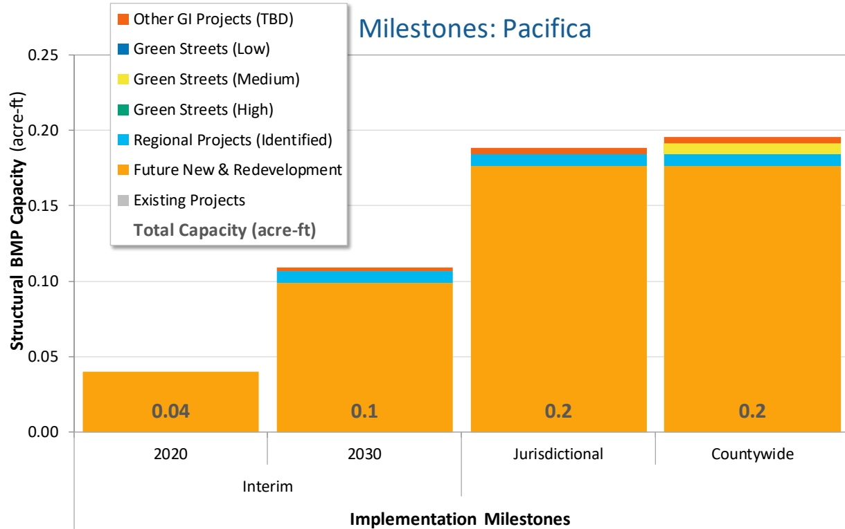
Figure 4-4. Summary GI Capacity for Interim and Final Implementation Milestones
