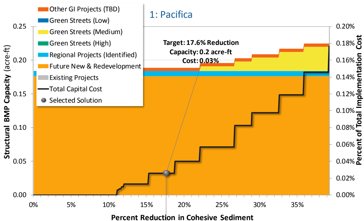
Figure 1-6. Scenario 1: Optimization summary for Pacifica (sediment target, with regional identified project).
