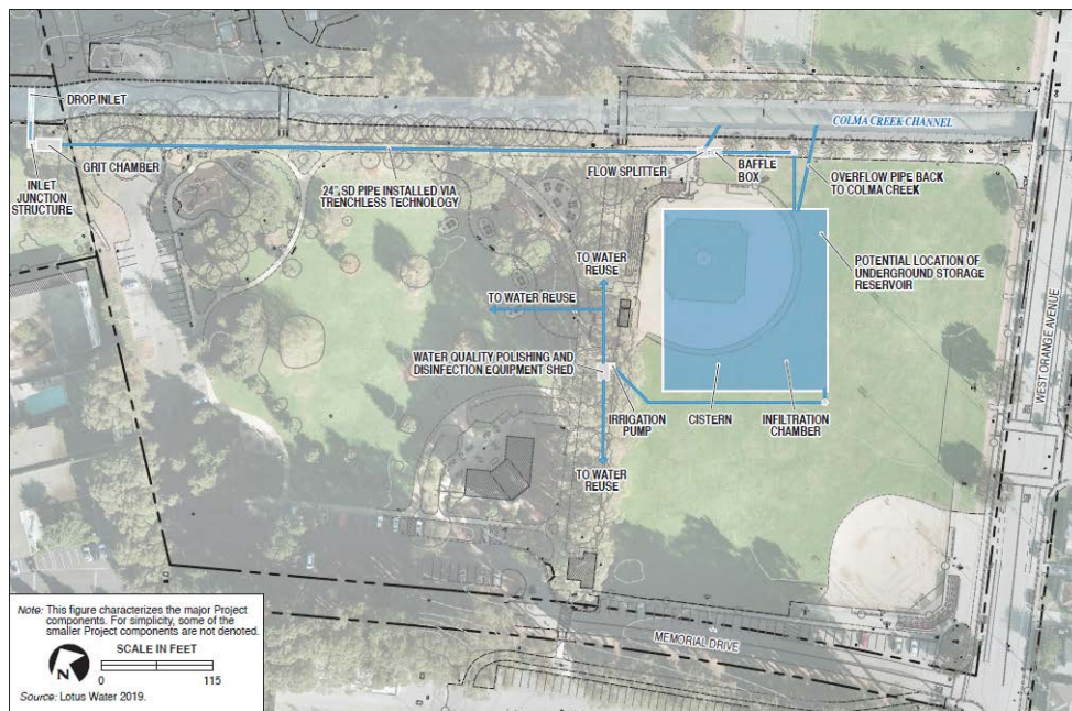
Figure 4-7. Concept for Orange Memorial Park Storm Water Capture Project
