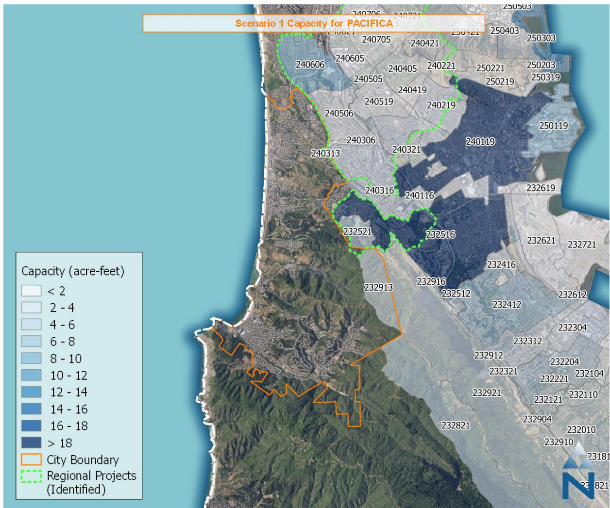
Figure 4-3. Map of GI capacities within each subwatershed of Pacifica
