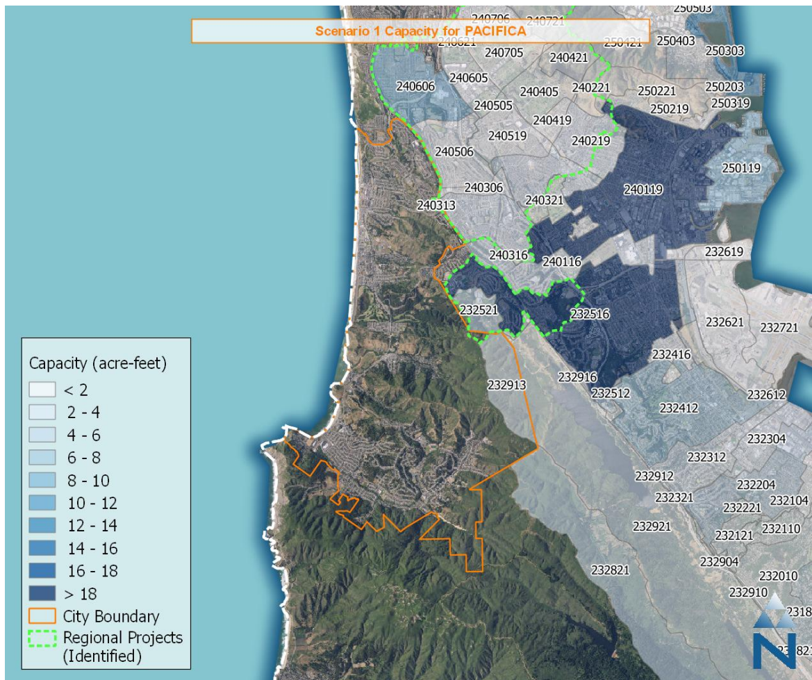
Figure 1-7. Scenario 1: Map of GI capacities within each subwatershed of Pacifica (sediment target, with regional identified project).
